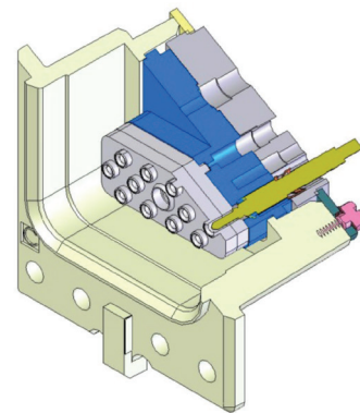
Custom Avionics Connector -787 Wing Engine Breakaway connector
