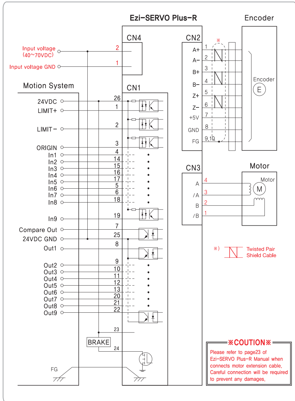
CONTROLLER EMBEDDED DRIVE EXTERNAL WIRING DIAGRAM(86mm Motor)
