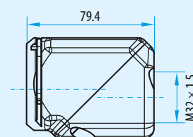
Straight cable exit
