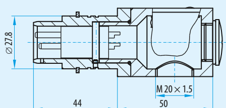
Pin piece
