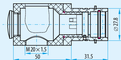
Socket piece
