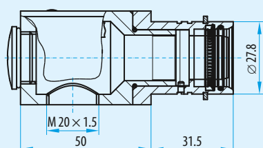
Socket piece
