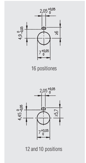
SK 20 · Mounting layouts
