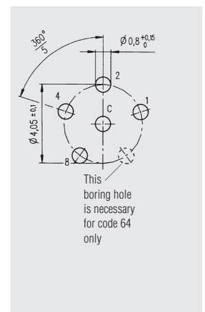
SK 20 · Hole location diagram
