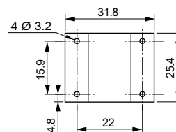
Bride BR001
