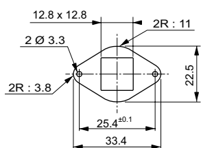
Joint JT001
