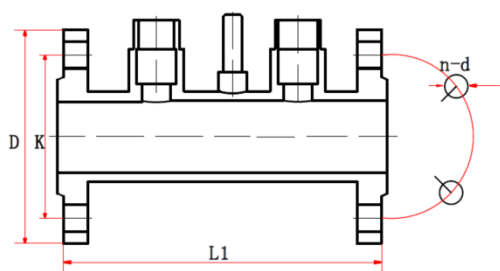
DN25-DN300 Flange connection Dimensions
