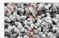
Standard compound, 6 µm diamond grit – poorly calibrated with uneven grit shape –
