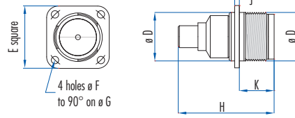
Panel connector
