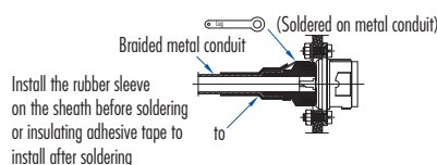
Panel connectors
