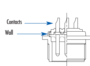
Square panel connector
