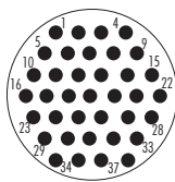
Housing 2 37 x \varnothing 1 mm
