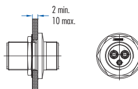
Bulkhead connector
