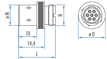
Coupler connector
