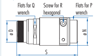
Coupler connector
