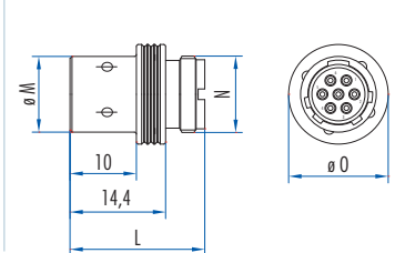
Coupler connector
