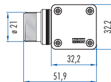
Coupler connector
