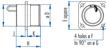
Panel connector
