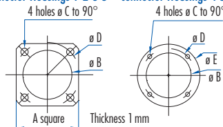
Square gasket under panel connector Housings 1-2-3-5
