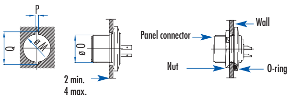
Diagram 1: Thickness of the wall between 2 and 4 mm
