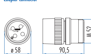
Coupler connector
