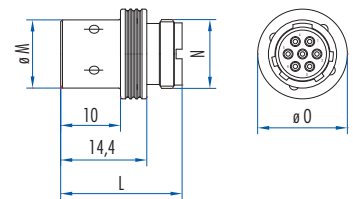
Coupler connector
