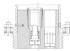
Panel connector
