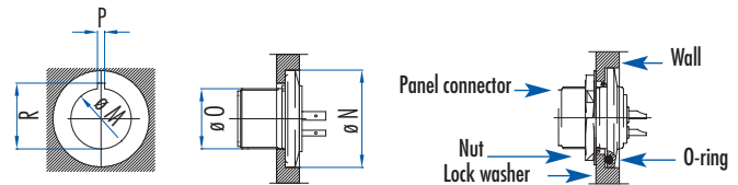
Diagram 2: Thickness of the wall greater than 4 mm
