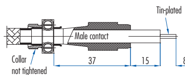
Panel connectors
