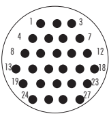
Housing 2 27 x \varnothing 1 mm
