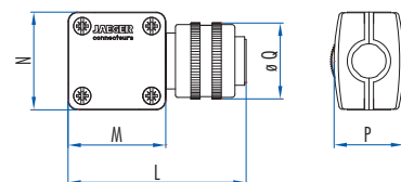
Cable connector
