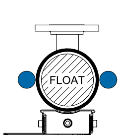
Probe mounting positions on Atlas™, Vector™, and Gemini™ Magnetic Level Indicators
