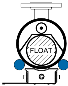
Probe mounting positions on Aurora® MLI Probe proximity to the float is critical
