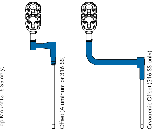
Sensor Enclosures (shaded) refer to Model Code digit 6
