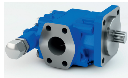
Optional Rickmeier product for Diesel engines: Fuel oil pump: R35/50 Appr. 70 dm 3 /min @ 1800 rpm Working pressure: 13 bar (max. 25 bar) Suction pressure: 0.6 bar abs. Kin. Viscosity: 4 mm 2 /s
