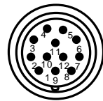
Pin plug 12-pin: Metal: RC-12P2N1280EF Plastic: RC-12P1N12K0EF
