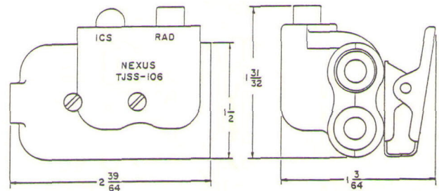
TJSS-106 TELEPHONE JACK, TWO SWITCHES BIAXIAL SHIELDED
