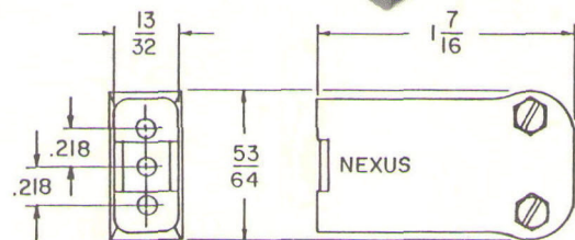
MJ-123 THREE CONDUCTOR JACK
