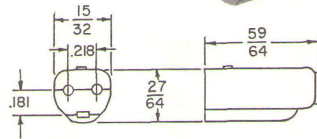
MJ-103 MICROPHONE LOCKING JACK, THREE CONDUCTOR
