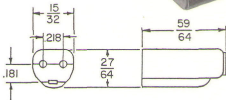
MJ-113 MICROPHONE JACK, THREE CONDUCTOR
