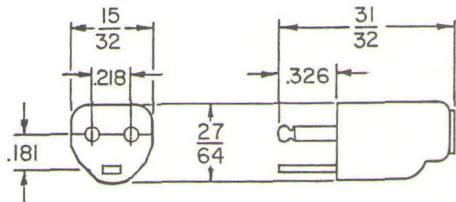
MP-103 MICROPHONE PLUG, THREE CONDUCTOR
