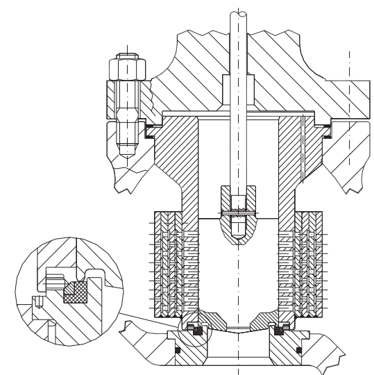
Fig. 11 Quick-change seat – Soft seat insert – Unbalanced trim
