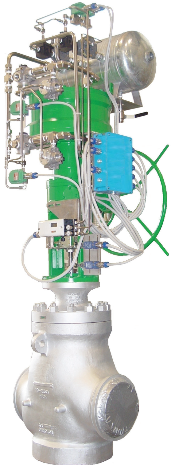
Fig. 1 Tecnoil Valve Model LN/L Globe Valve 10" ANSI 300 with pneumatic actuator
