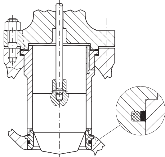
Fig. 10 Quick change seat, Unbalanced trim
