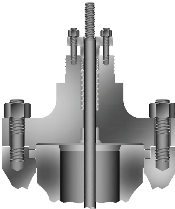
Fig. 4 Standard bonnet
