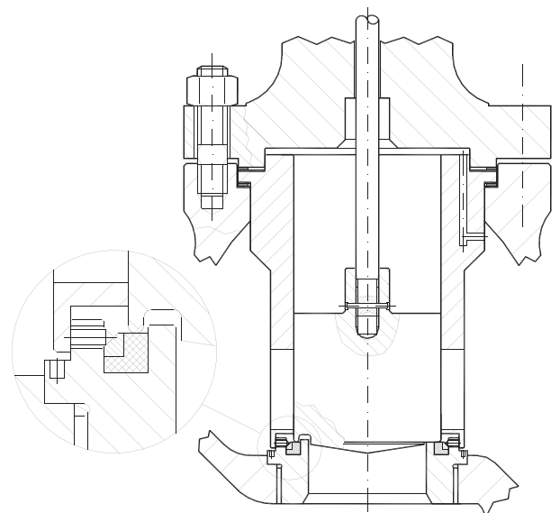
Fig. 7 Threaded seat – Soft seat insert – Unbalanced trim
