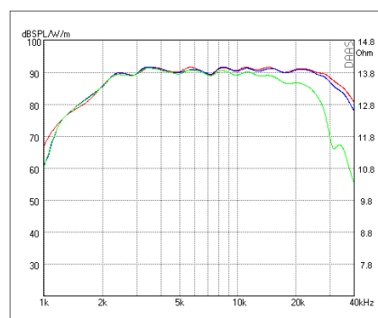
SPL Vertically 0° - 5° - 15°
