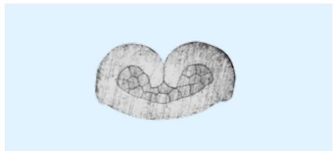
The F crimp results in a well-defined, clean pinch.
