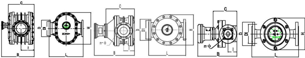
➤ LC-A Cast Iron Oval Gear Flow meter Dimensions (B=Register A dimensions) Unit :mm
