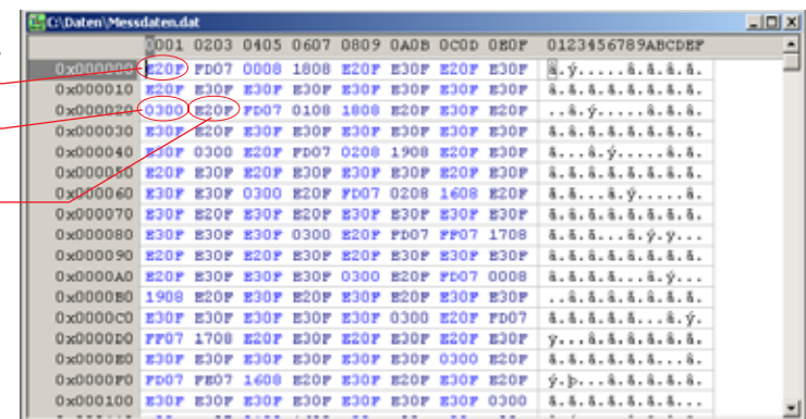
Sample file shown with a Hex Viewer
