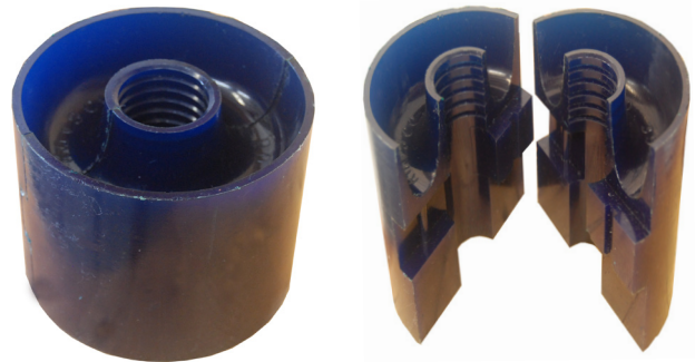
Unique Design Split Seals - Easy installation for umbilical diameters: 4 mm - 76 mm
