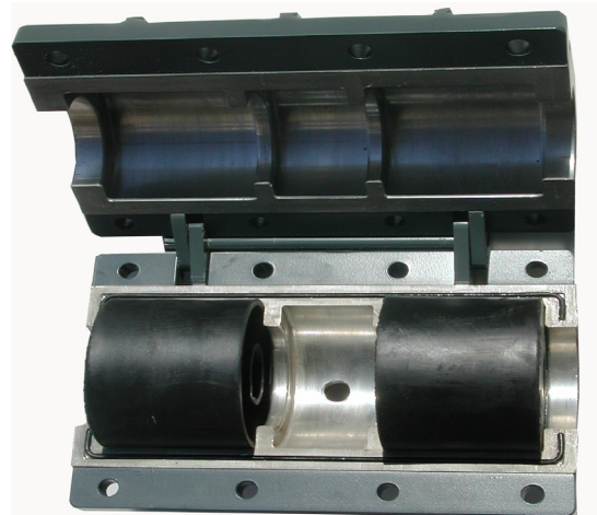
Unique Design Split Seals - Easy installation for umbilical diameters: 4 mm - 76 mm
