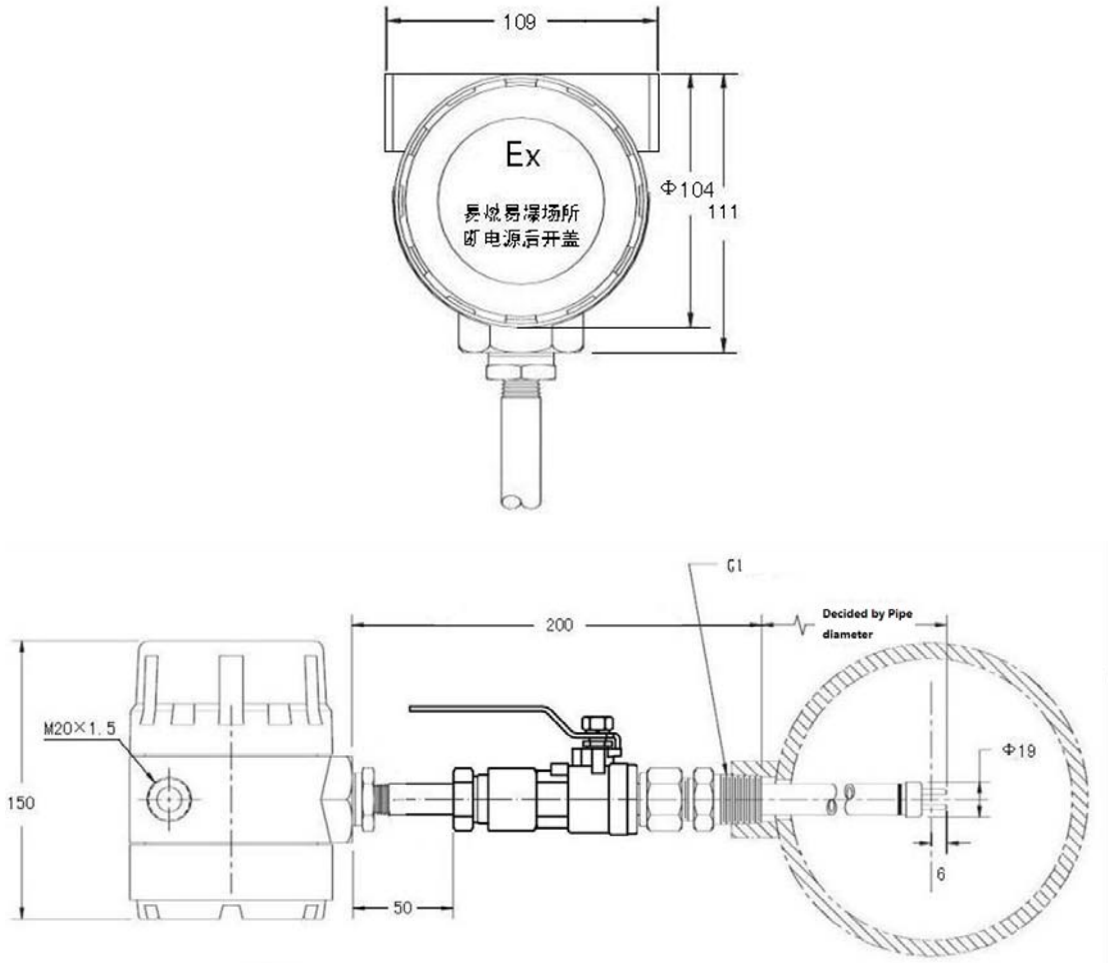
Figure 1: Dimension of Thermal Mass Flow meter
