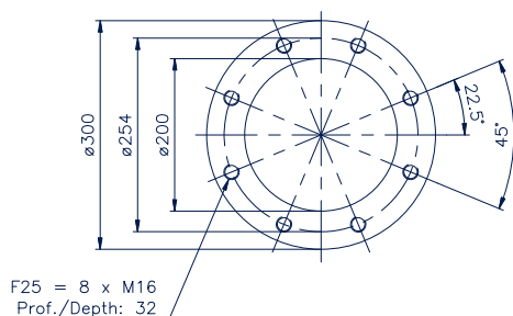
Vue A de la bride View A of the flange
