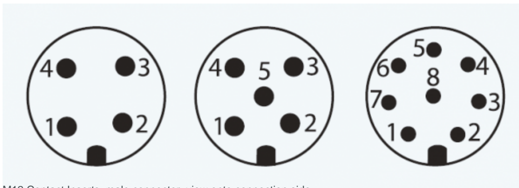
M12 Contact Inserts, male connector, view onto connection side
