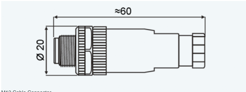
M12 Cable Connector
