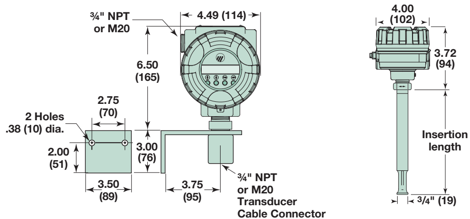
Remote Mount Model TA2
