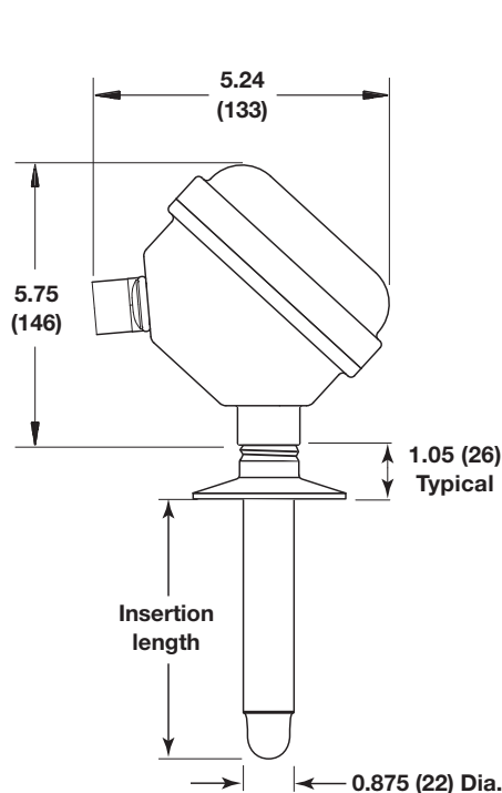
Model TD2 with Hygienic Housing Tri-Clamp® Connection
