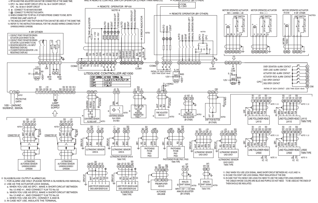
Liteguide Controller Model AE1000 (for CPC) Dwg. no. MK0000030-EC2
