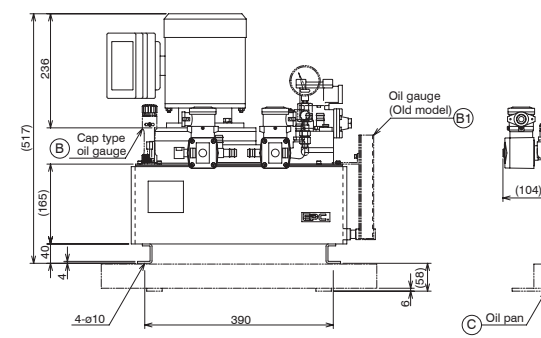
Servoguide MK-IV.D (Low-load type) (pressure-resistant explosion-proof) MODEL D053B(P)-AM-2 Drawing No. AD6862.0-20E D053B(P)-AM-3
