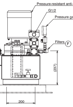
Servoguide MK-IV.D (Low-load type) (pressure-resistant explosion-proof) MODEL D053B(P)-AM-2 Drawing No. AD6862.0-20E D053B(P)-AM-3
