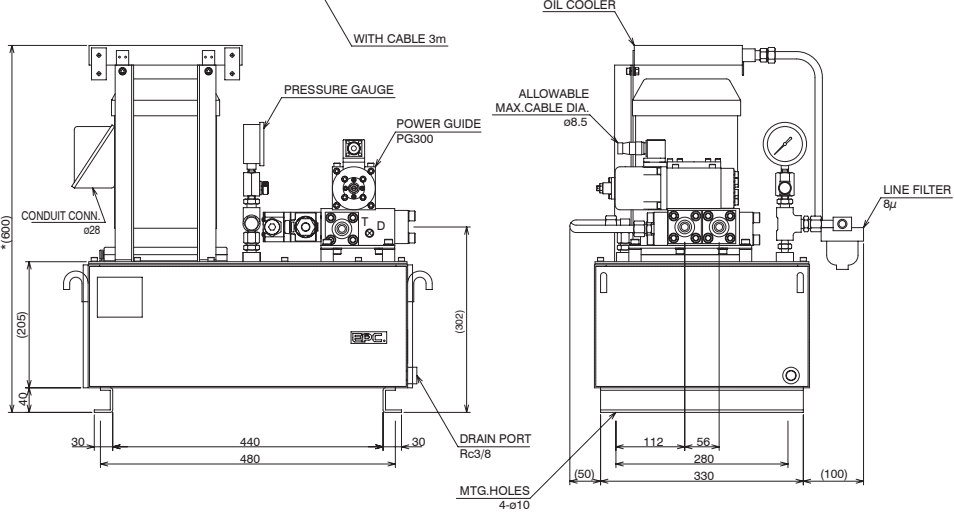
Power Guide Unit (High output/High response type) MODEL M820-AM Drawing No. AD000140-EA
