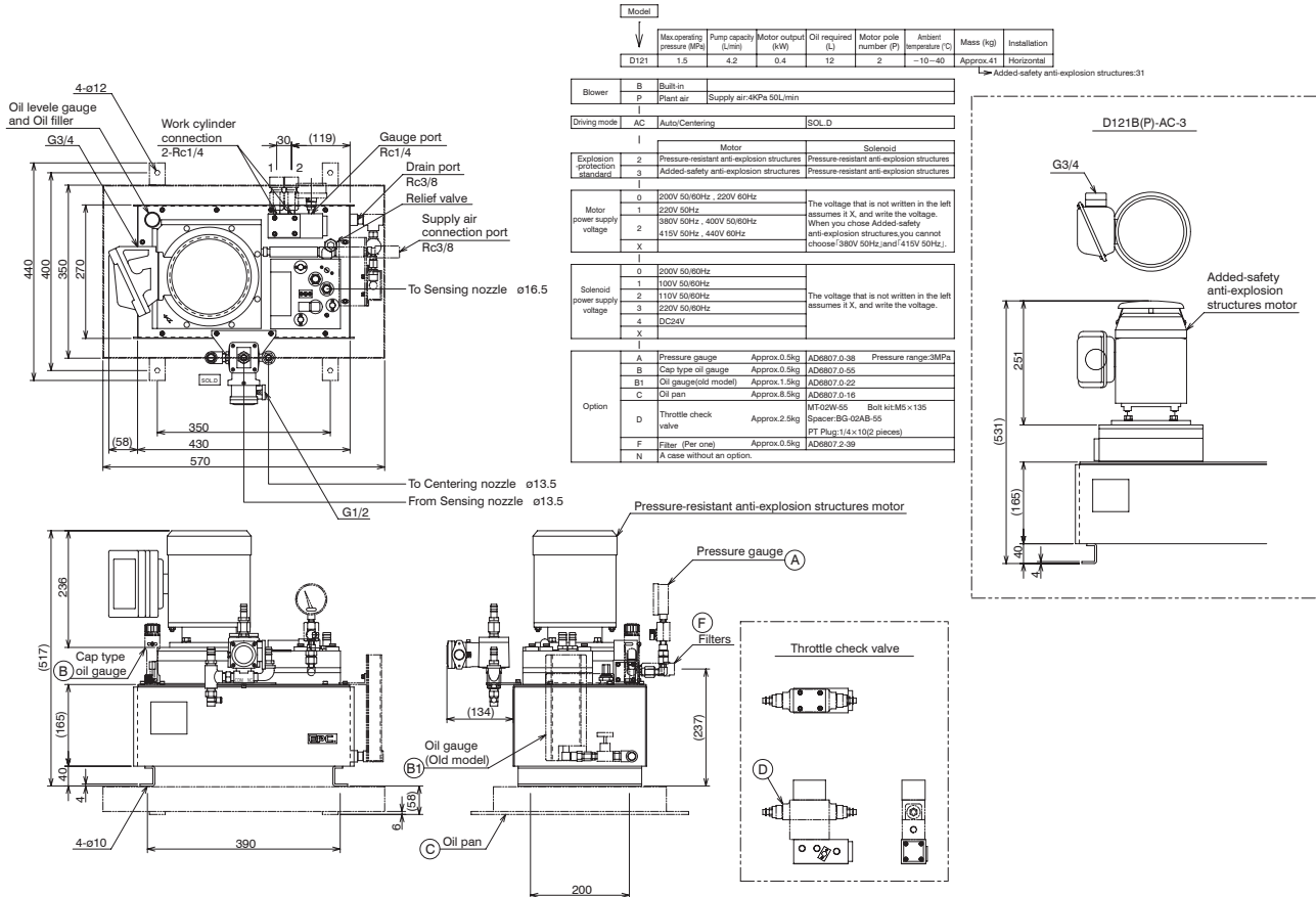
Servoguide MK-IV.D (Single type) (pressure-resistant explosion-proof) MODEL D121B(P)-AC-2 D121B(P)-AC-3 Drawing No. AD6864.0-40E
