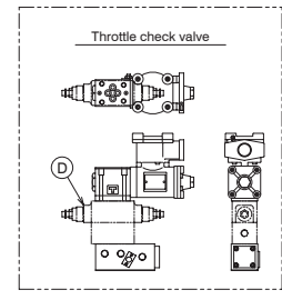
Servoguide MK-IV.D (Low-load type) (pressure-resistant explosion-proof) MODEL D053B(P)-AM-2 Drawing No. AD6862.0-20E D053B(P)-AM-3
