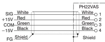
Photohead PH22VAS-R (Vacuum environment compatible) (cable exit to the back) Drawing No. MD0003080-EA
