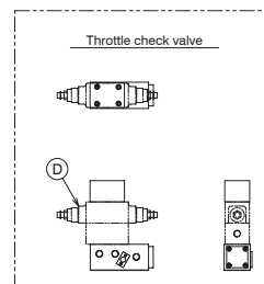
Servoguide MK-IV.D (Single type) MODEL D121B(P)-AC-0 D121B(P)-AC-1 Drawing No. AD6863.0-40E
