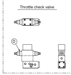
Servoguide MK-IV.D (Low-load type) MODEL D053B(P)-AC-0 D053B(P)-AC-1 Drawing No. AD6861.0-40E
