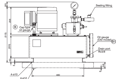
Servoguide MK-IV.M (High-load type) (explosion-proof type solenoid valve and motor) MODEL M721-AM-2 M721-AM-3 Drawing No. AD6860.0-20E
