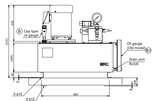
Servoguide MK-IV.M (High-load type) MODEL M721-AM-0 M721-AM-1 Drawing No. AD6859.0-20E
