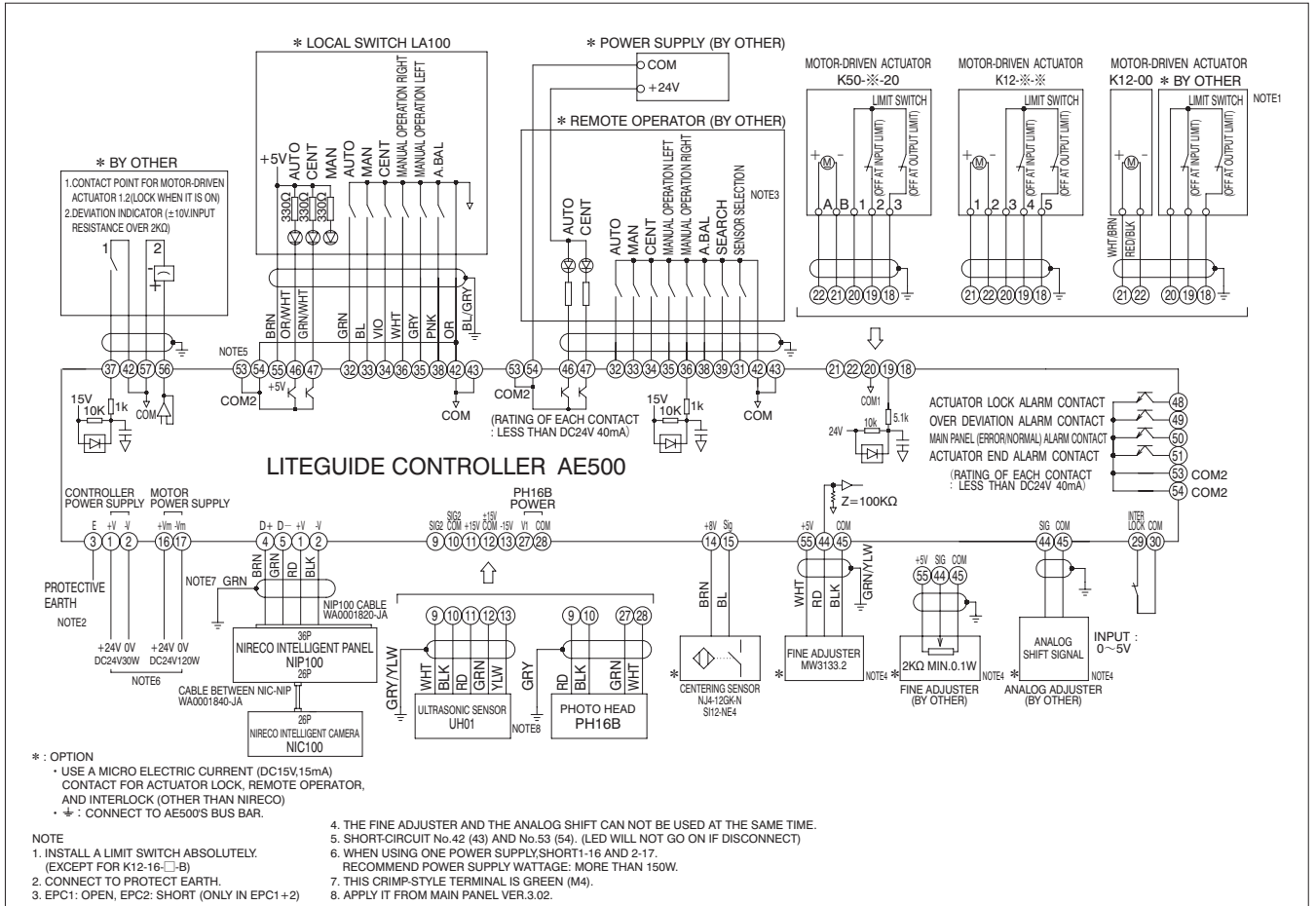
Liteguide Controller Model AE500 Wiring diagrams Drawing No. MK0001030-EC2
