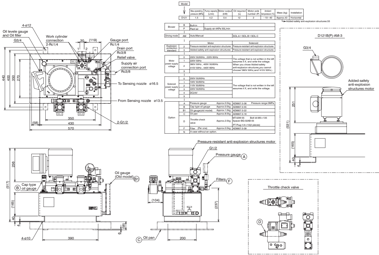
Servoguide MK-IV.D (Single type) (pressure-resistant explosion-proof) MODEL D121B(P)-AM-2 D121B(P)-AM-3 Drawing No. AD6864.0-20E
