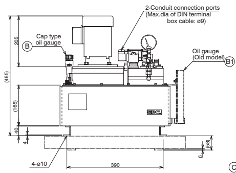
Servoguide MK-IV.D (Low-load type) MODEL D053B(P)-AM-0 D053B(P)-AM-1 Drawing No. AD6861.0-20E
