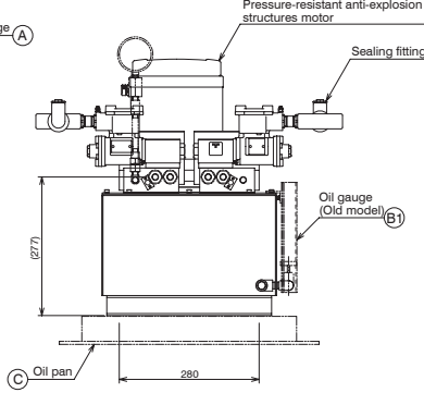
Servoguide MK-IV.M (Twin type) (explosion-proof type solenoid valve and motor) MODEL M220-AM-2 M220-AM-3 Drawing No. AD6858.0-20E
