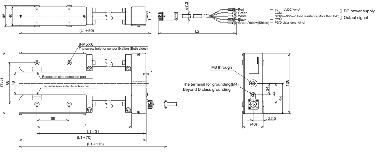
Ultrasonic Sensor UH01A (Extended sensor type) Drawing No. MD0365.0-EA
