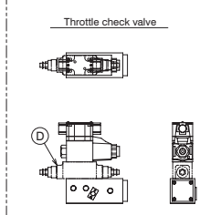
Servoguide MK-IV.D (High-load type) MODEL D721B-AM-0 Drawing No. AD6867.0-20E D721B-AM-1
