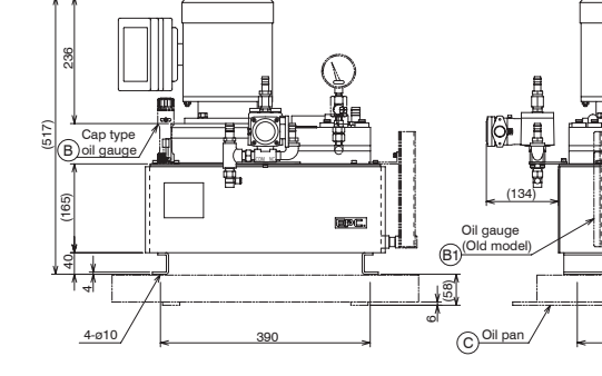
Servoguide MK-IV.D (Low-load type) (pressure-resistant explosion-proof) MODEL D053B(P)-AC-2 Drawing No. AD6862.0-40E D053B(P)-AC-3
