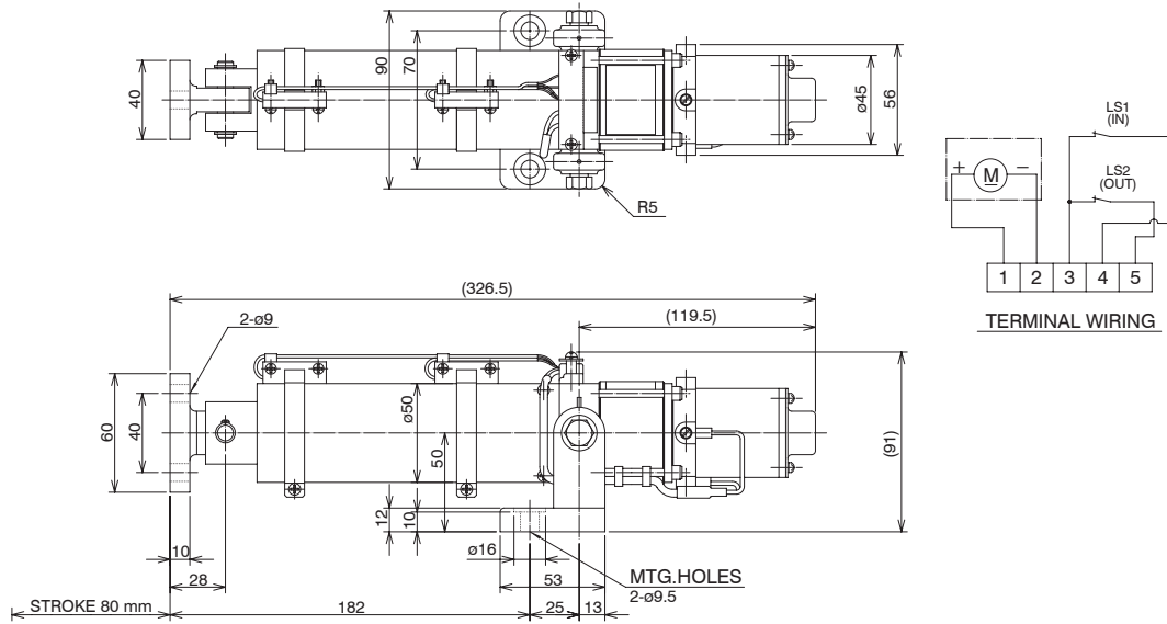
Motor-driven actuator K12-80-20 Drawing No. KL9034.0-EA
