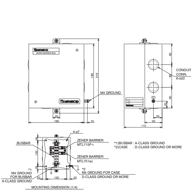
Zener barrier box intrinsic safety construction Ultrasonic Sensor Drawing No. MW9013.0-EA
