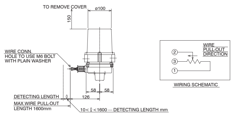
Photohead PH30N (No air purge) PH30P (with air purge) Drawing No. MD0134.1-EA
