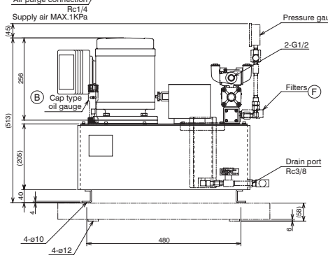
Servoguide MK-IV.M (Twin type) (explosion-proof type solenoid valve and motor) MODEL M220-AM-2 M220-AM-3 Drawing No. AD6858.0-20E
