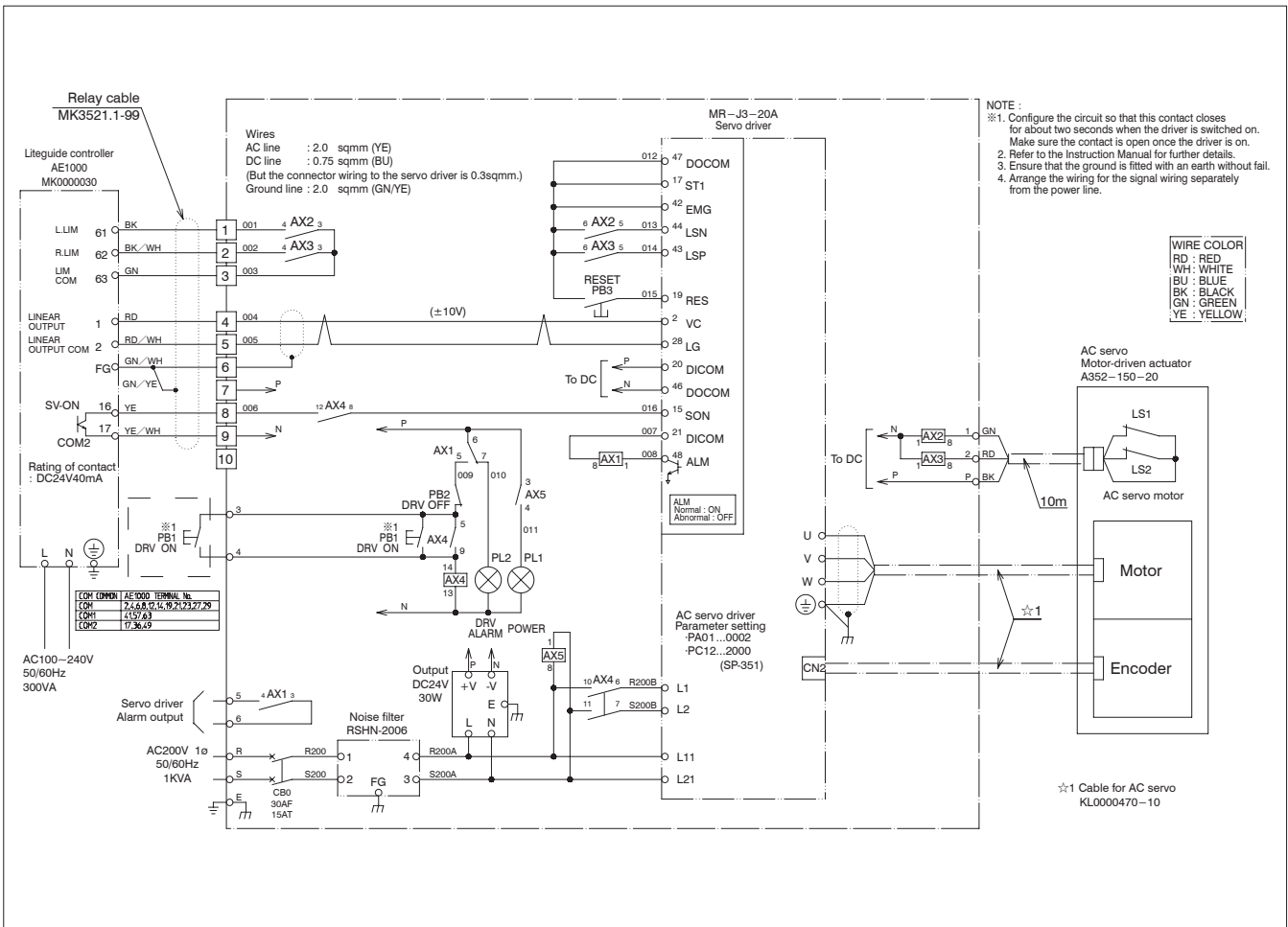
AC servo driver unit SP-351/A352 Drawing No. MK3521.3-EC3
