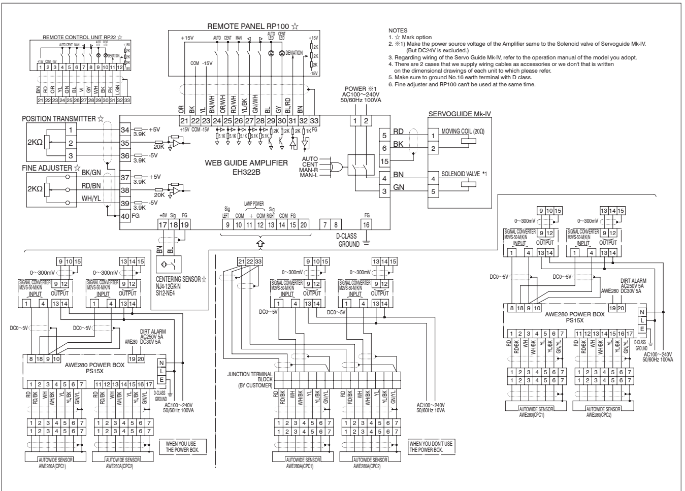
Webguide Amplifier EH322B Drawing No. MK0003280-EC1
