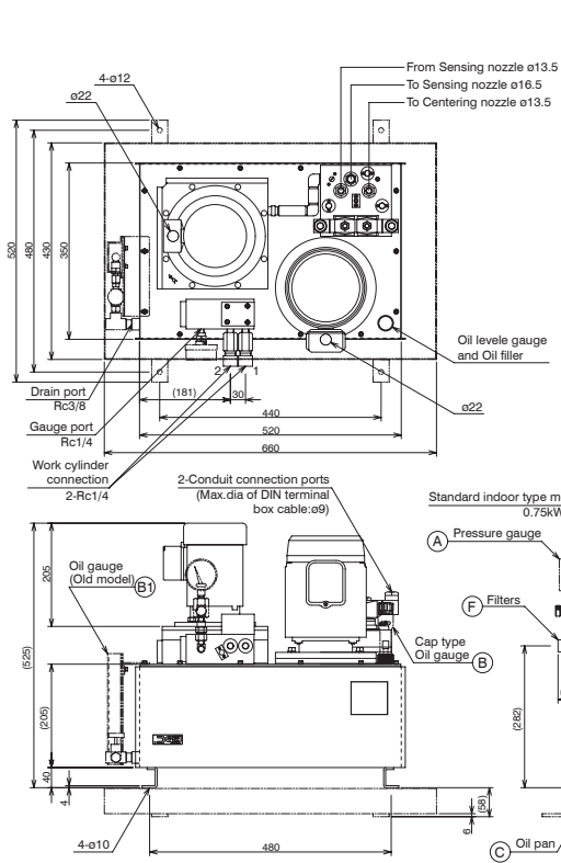
Servoguide MK-IV.D (High-load type) MODEL D721B-AC-0 Drawing No. AD6867.0-40E D721B-AC-1
