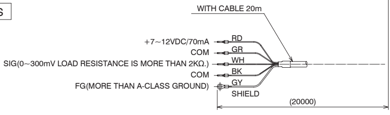
Ultrasonic Sensor UH01 UH01S (with screw guider) (intrinsically safe anti-explosion systems) Drawing No. KL0000670-EA Drawing No. KL0000700-EA
