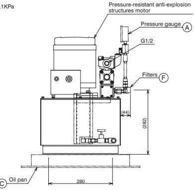
Servoguide MK-IV.M (High-load type) (explosion-proof type solenoid valve and motor) MODEL M721-AM-2 M721-AM-3 Drawing No. AD6860.0-20E
