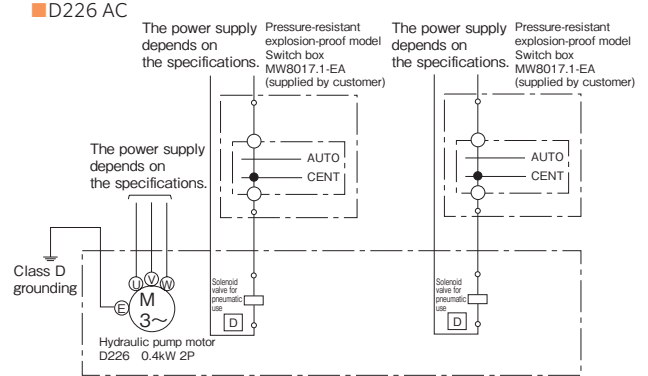
Servoguide D models (standard)
