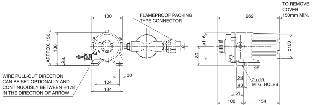
Analog position transmitter wire position sensor FW31 Drawing No. MW1102.2-EA
