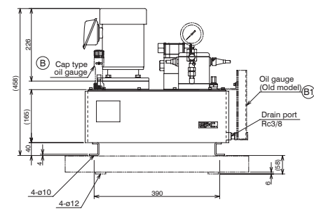
Servoguide MK-IV.M (Single type) MODEL M121-AM-0 M121-AM-1 Drawing No. AD6855.0-20E
