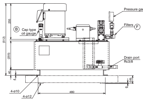
Servoguide MK-IV.M (Twin type) MODEL M220-AM-0 M220-AM-1 Drawing No. AD6857.0-20E
