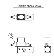
Servoguide MK-IV.D (High-load type) MODEL D721B-AC-0 Drawing No. AD6867.0-40E D721B-AC-1
