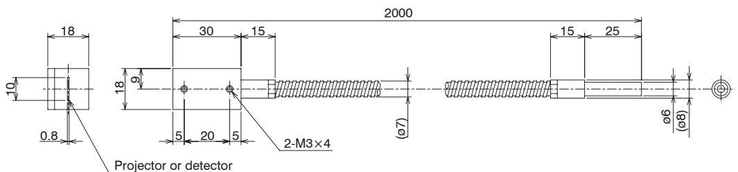
High-temperature EPC sensor HE120A Drawing No. MD0408.1-EA
