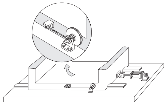
Mounting diagram
