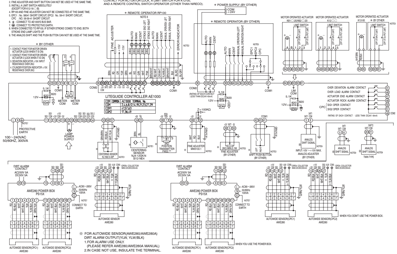
Liteguide Controller Model AE1000 (for CPC) Drawing No. MK000030-EC4
