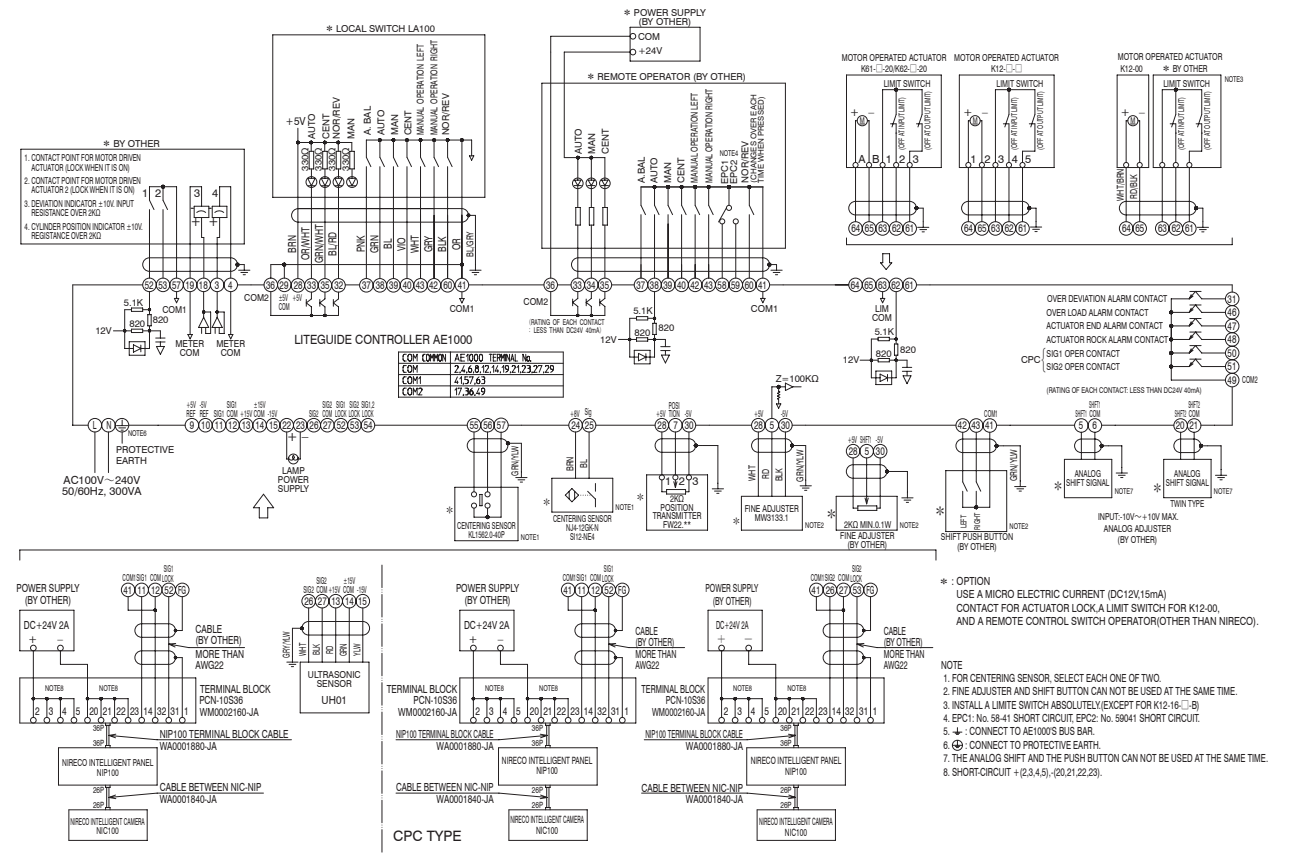
Liteguide Controller Model AE1000 (for DPC) Dwg. no. MK0000030-EC3
