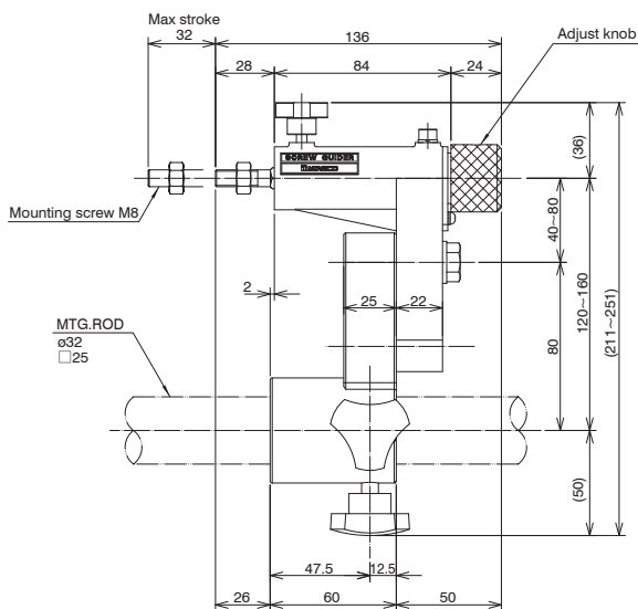
Screw Guider Drawing No. KL0000570-EA
