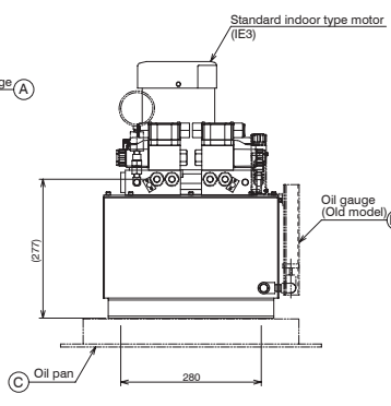
Servoguide MK-IV.M (Twin type) MODEL M220-AM-0 M220-AM-1 Drawing No. AD6857.0-20E
