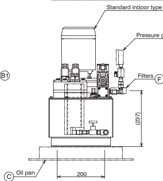
Servoguide MK-IV.D (Single type) MODEL D121B(P)-AM-0 D121B(P)-AM-1 Drawing No. AD6863.0-20E
