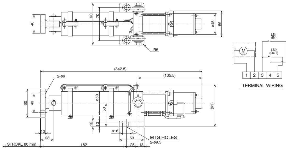
Motor-driven actuator K12-80-07 Drawing No. KL9033.0-EA
