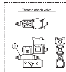
Servoguide MK-IV.D (High-load type) (pressure-resistant explosion-proof) MODEL D721B-AM-2 D721B-AM-3 Drawing No. AD6868.0-20E
