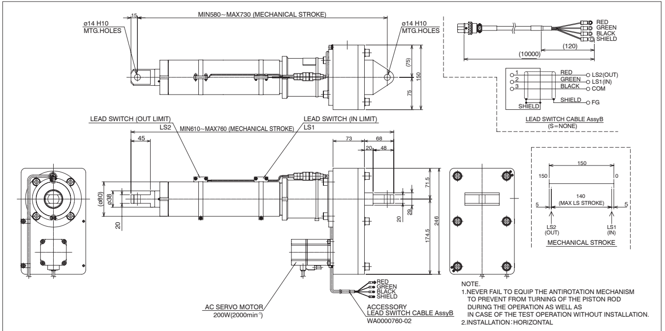
AC servo actuator A352-150-20 Drawing No. KL0000630-EA
