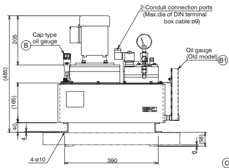
Servoguide MK-IV.D (Low-load type) MODEL D053B(P)-AC-0 D053B(P)-AC-1 Drawing No. AD6861.0-40E
