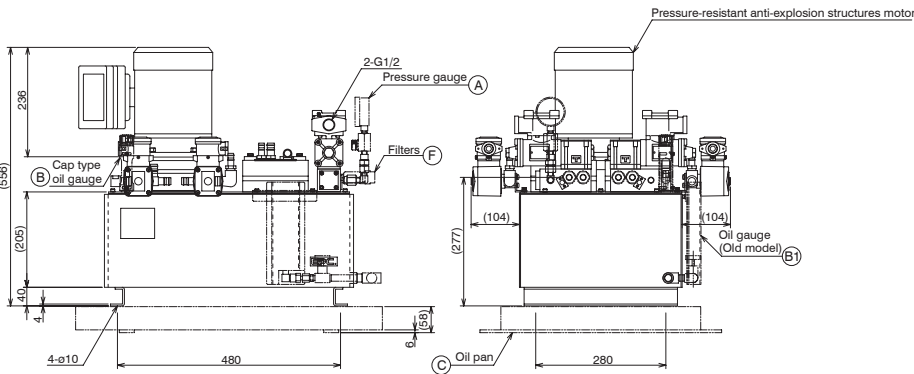
Servoguide MK-IV.D (Twin type) (pressure-resistant explosion-proof) MODEL D226B(P)-AM-2 D226B(P)-AM-3 Drawing No. AD6866.0-20E
