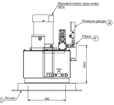
Servoguide MK-IV.M (High-load type) MODEL M721-AM-0 M721-AM-1 Drawing No. AD6859.0-20E
