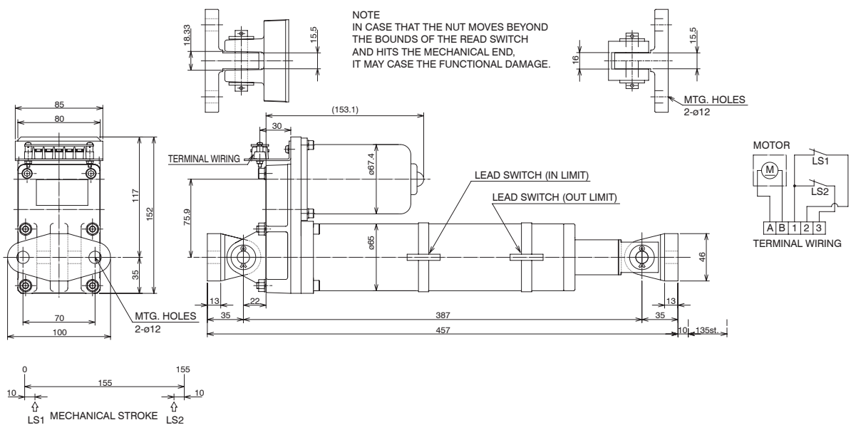
Motor-driven actuator K62-150-20 Drawing No. KL0000450-EA
