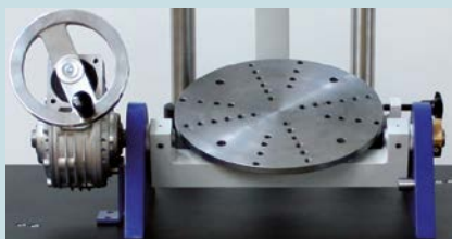
Clamping table DS 300 with clamping plate Ø 300 mm
