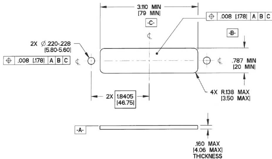
Recommended Plug Panel Cutout Dimensions
