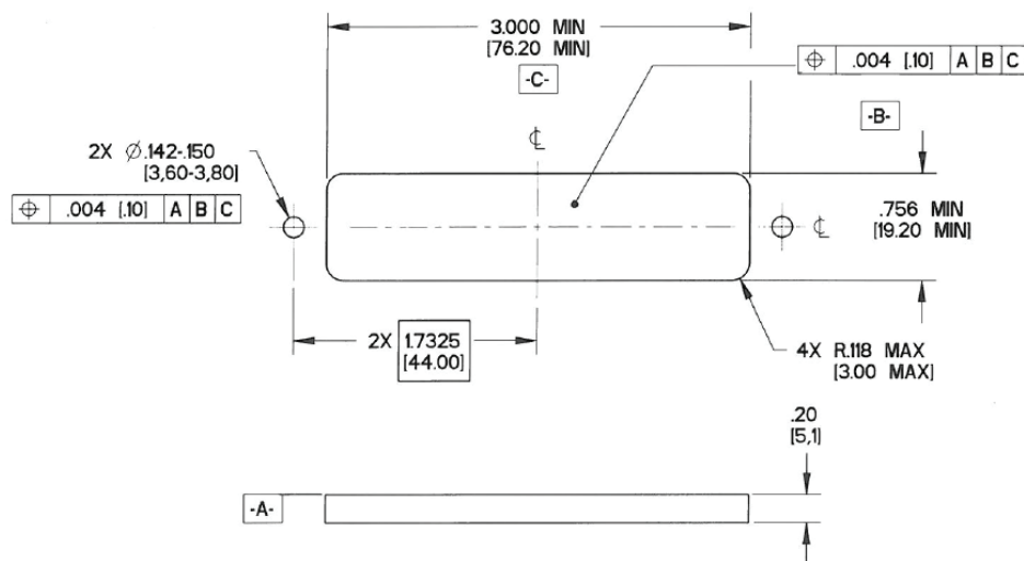
Recommended Receptacle Panel Cutout Dimensions
