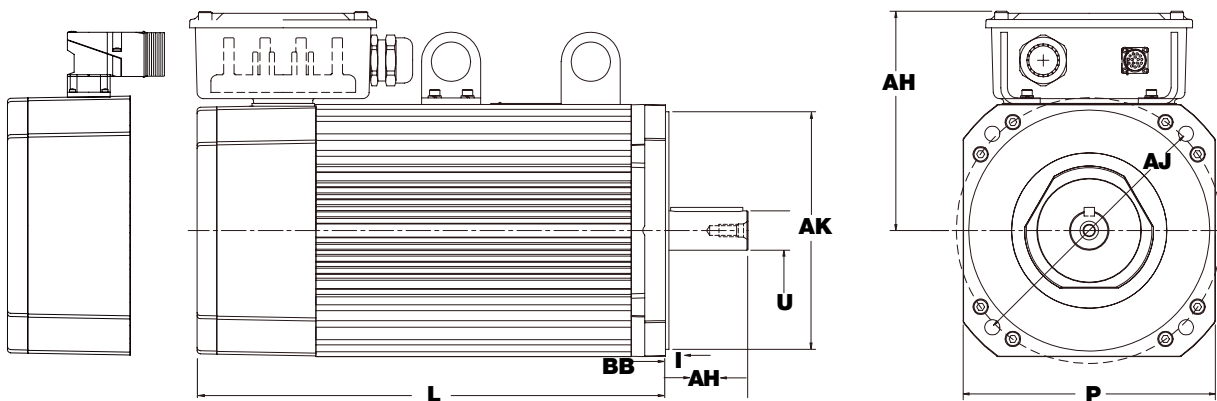
Rotatable Connector
