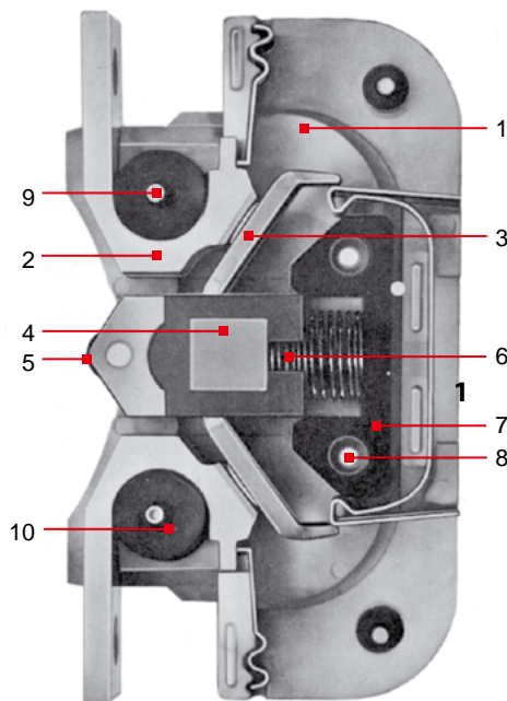
Section through a cam-operated switching element with mounted arc chamber
