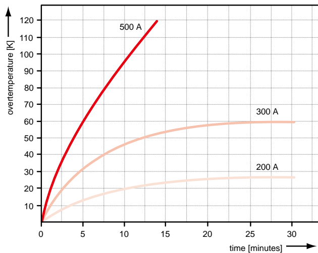
Temperature rise of switching element S307 A and S307 C resp. (wire cross section area 95 mm 2 ) The permissible conventional thermal current for this series is 300 A (contact pressure 10 N).
