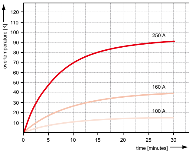
Temperature rise of switching element S306 K and S306 M resp. (wire cross section area 35 mm 2 ) The permissible overtemperature is only reached at an amperage of over 160 A. The permissible conventional thermal current is 160 A (contact pressure 3.5 N).
