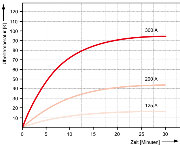
Temperature rise of switching element S306 A and S306 C resp. (wire cross section area 50 mm 2 ) The permissible conventional thermal current for this series is 200 A (contact pressure 5.5 N).
