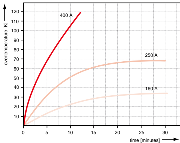
Temperature rise of switching element S307 E and S307 G resp. (wire cross section area 70 mm 2 ) The permissible conventional thermal current for this series is 250 A (contact pressure 5.5 N).
