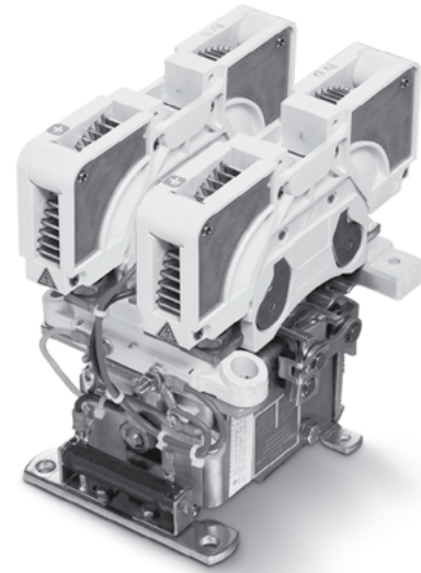
C155 P Series contactor: Fitted with cam-operated switching element S307 C /N and arc chute LK-S307-DC.
