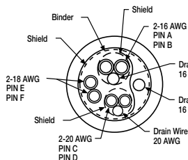
Cable End View
