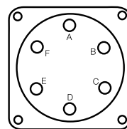
MOTOR CONNECTOR MS3102E-14S-06P
