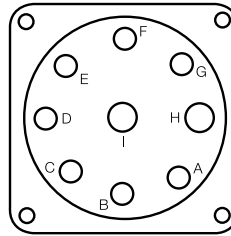
MOTOR CONNECTOR MS3102E-20-16P
