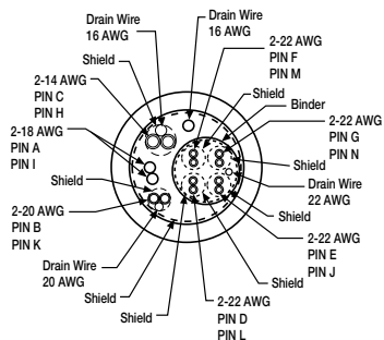
Cable End View
