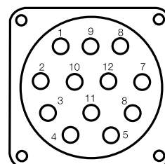
MOTOR CONNECTOR CHROME 12 PIN
