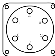
MOTOR CONNECTOR MS3102E-14S-06P
