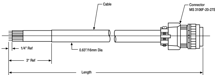
M2200/3300 Cable Assembly
