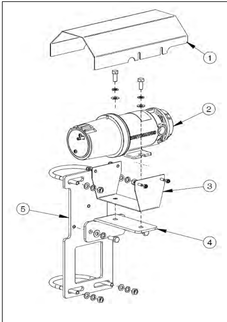
Vertical Mount
