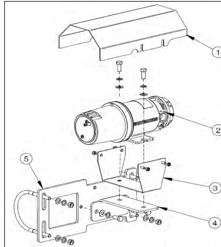
Horizontal Mount
