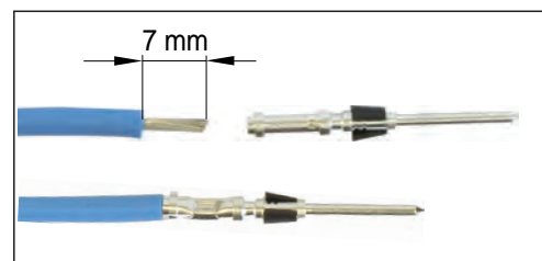
Fig. 11: Skin cable strands and crimp to contacts.
