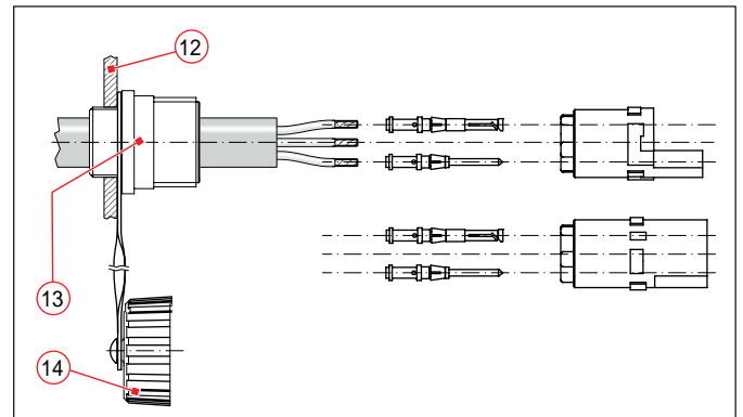
Fig. 10: Example of assembly for receptacles with thread on a mounting wall (applies also for plugs with thread)
