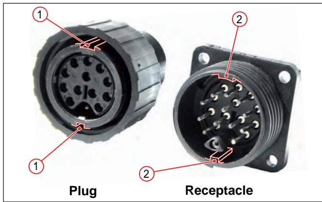
Fig. 24: Series M3: Grooves (1) on plug and guideways (2) on receptacle
