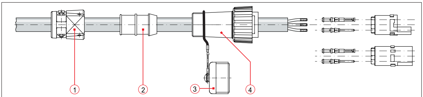
Fig. 6: Example for cable plug with back shell, strain relief and cable gland (applies also for cable receptacles)
