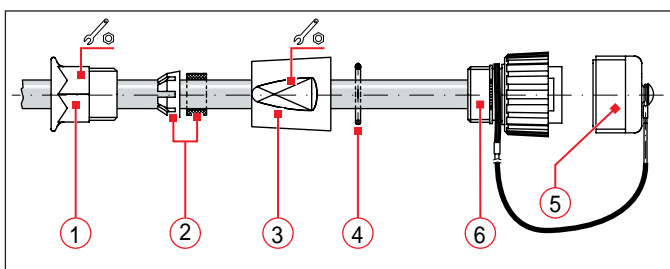
Fig. 21: Example for plug with thread, back shell and cable gland (applies also for receptacles with thread)
