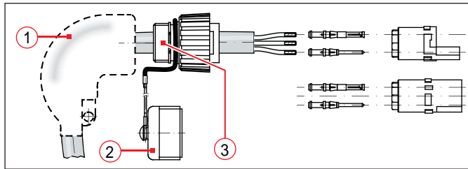
Fig. 8: Example for plug with threaded rear skirt and 90° shrink boot (applies also for receptacles with thread)
