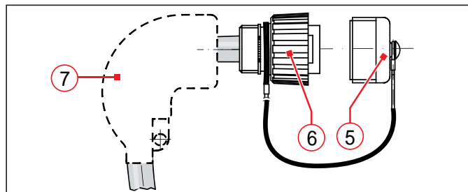
Fig. 22: Example for plug with thread and 90° shrink boot (applies also for receptacles with thread)
