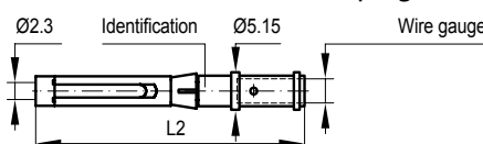
Socket contact
