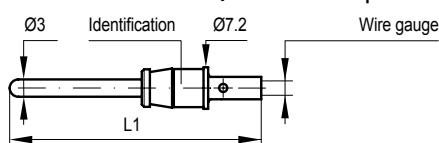
Pin contact
