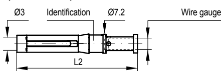
Socket contact
