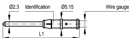
Pin contact
