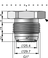
CG1-S38 type G1" with flush diaphragm
