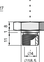
G1/4" type
