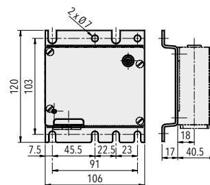
Mounting plate MB31 see chapter 'Accessories'
