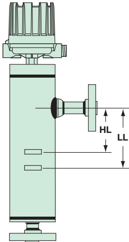
Sealed Chamber Side/Bottom Flange Connections (B74, H13, H31, H51)
