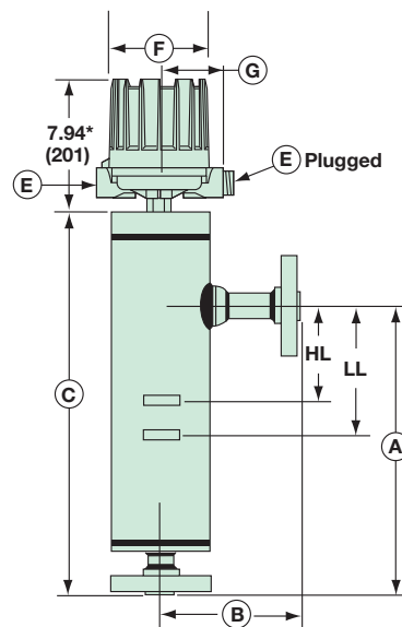
Sealed Chamber Side/Bottom Flange Connections (B74, H13, H31, H51)
