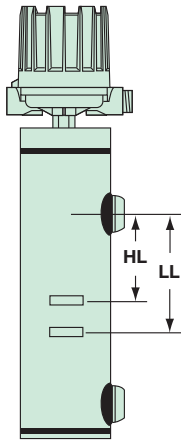
Sealed Chamber w/NPT or Socket weld Side/Side Connections (H13, H31, H51)
